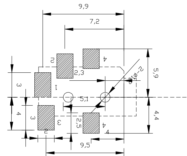
HOLE LAYOUT
