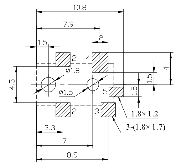
HOLE LAYOUT
