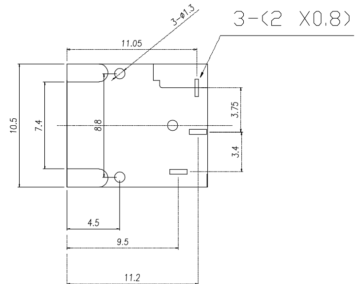
HOLE LAYOUT
