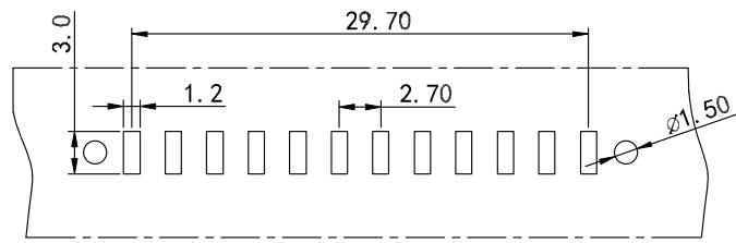
RECOMMENDED PCB LAYOUT T=0.65MM, TOLERANCES ±0.05MM
