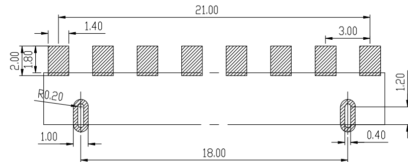
RECOMMENDED PCB LAYOUT TOL:(±0.05)
