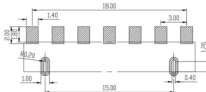
RECOMMENDED PCB LAYOUT TOL:(±0.05)
