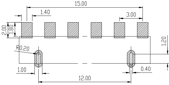
RECOMMENDED PCB LAYOUT TOL:(±0.05)
