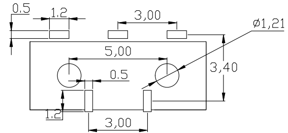
RECOMMENDED PCB LAYOUT TOL:(±0.05)
