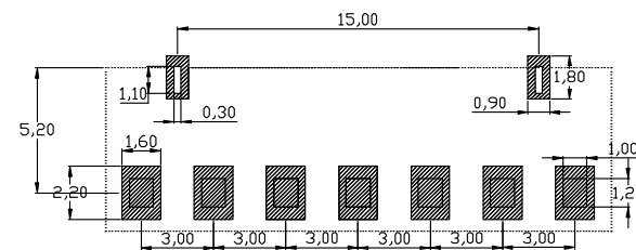
RECOMMENDED PCB LAYOUT TOP VIEW (.XX±0.05)
