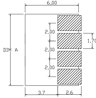
RECOMMENDED PCB LAYOUT TOP VIEW(.XX±0.05)
